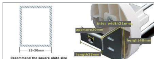
SF3001-SQUARE TUBE
