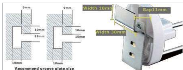
SF2002-GROOVE PLATE
