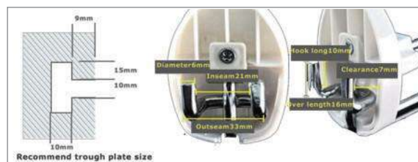
SF2001-SLOT PLATE
